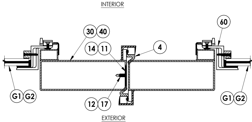
3 6 HORIZONTAL CROSS SECTION Outswing Shown (Inswing Similar)
