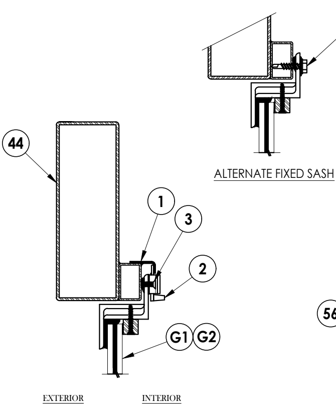
2/3 VERTICAL CROSS SECTION
