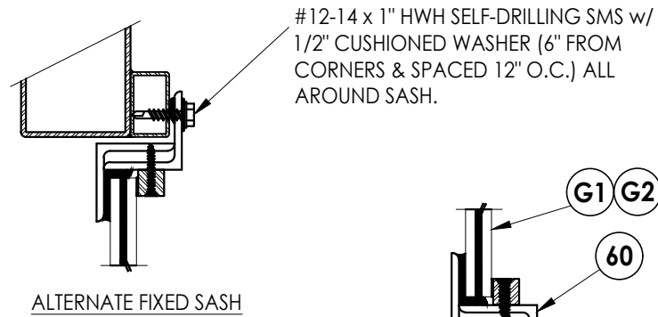
ALTERNATE FIXED SASH
