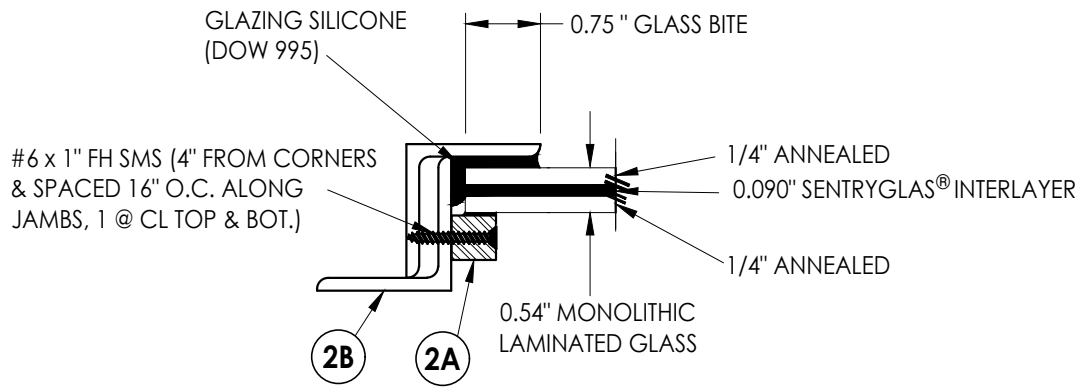
G1 GLAZING DETAIL Operable Door/Sidelite
