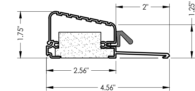
26 OUTSWING THRESHOLD
