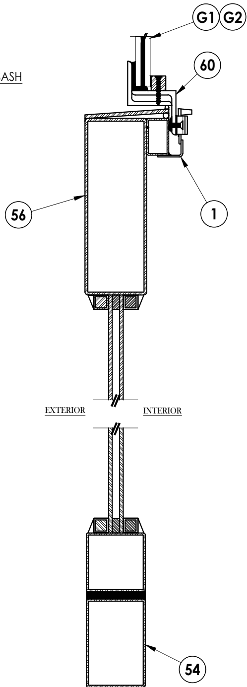
4/3 VERTICAL CROSS SECTION
