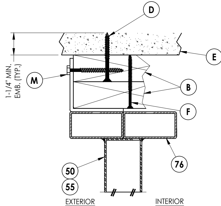
3 7 VERTICAL CROSS SECTION Outswing Shown (Inswing Similar)
