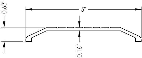
27 ADA THRESHOLD
