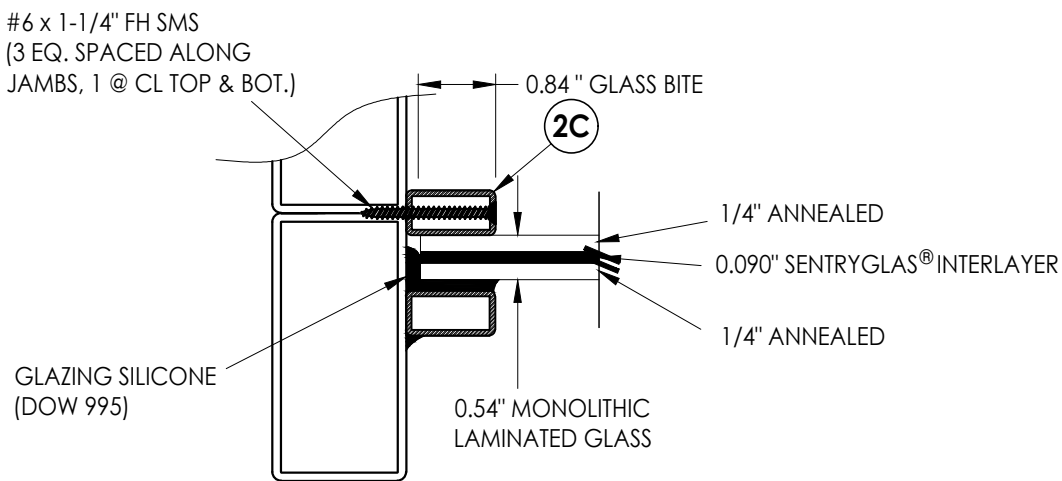
G1 GLAZING DETAIL Fixed Sidelite/Transom
