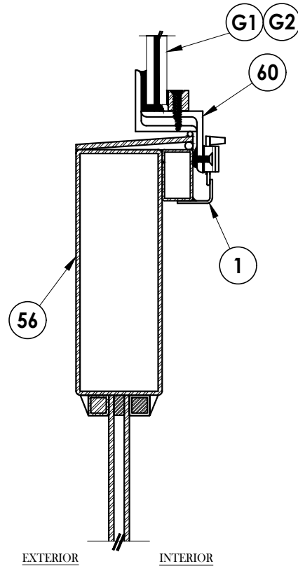
ALTERNATE FIXED SASH
