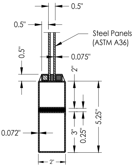
54 Bottom Rail 3/4 Lite Sidelite Panel
