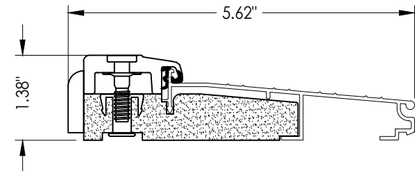
28 INSWING THRESHOLD
